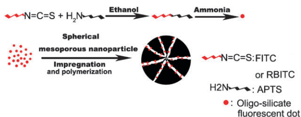
Scheme 1 A novel doping procedure for dyes into monodisperse mesoporous silica particles.
