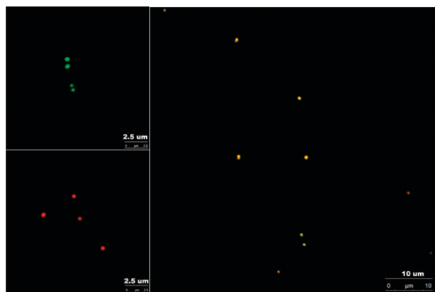
Fig. 3 Confocal fluorescence images of MSPs with different doping ratios between FITC and RBITC under 488 nm argon ion laser excitation: (a) 1 : 0; (b) 0 : 1; (c) 1 : 1.
