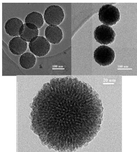
Fig. 1 TEM images of spherical mesoporous silica nanoparticles.
